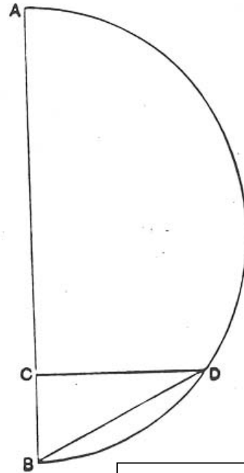
Diagram 10: Icosahedran (Heath)
