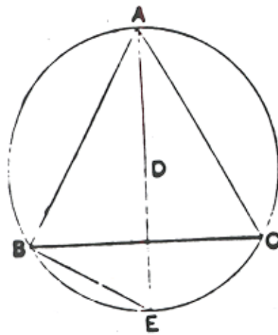
Diagram 5
