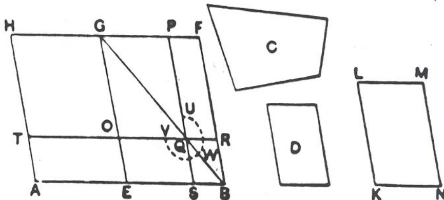
Diagram 3: Book 6, Prop 28
