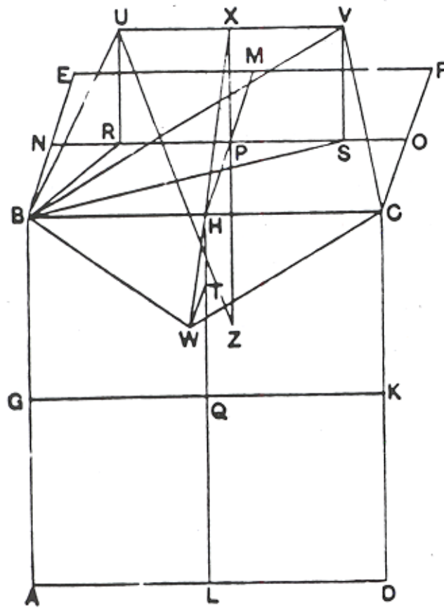
Diagram 12: Dodecahedron
