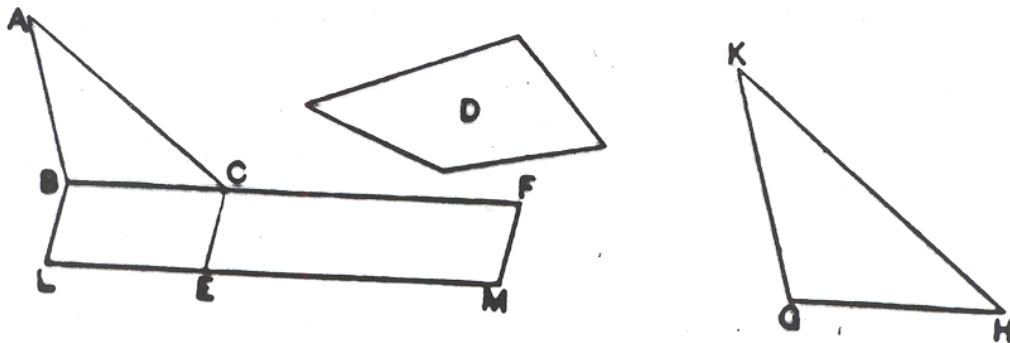
Diagram 2: Book 6, Props 28, 29
