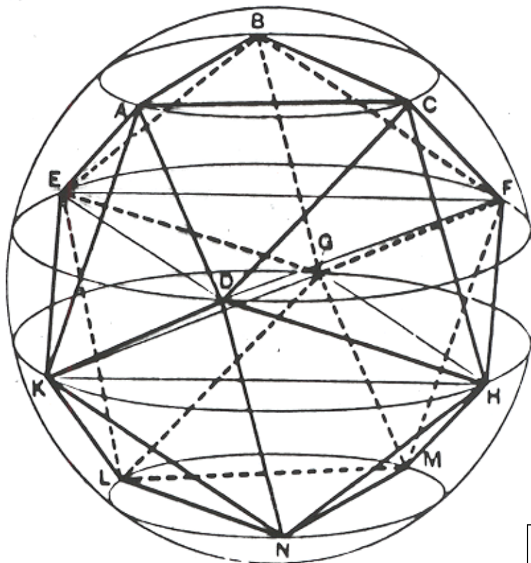
Diagram 11: Icosahedron (Pappus)
