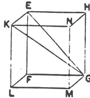
Diagram 8: Cube
