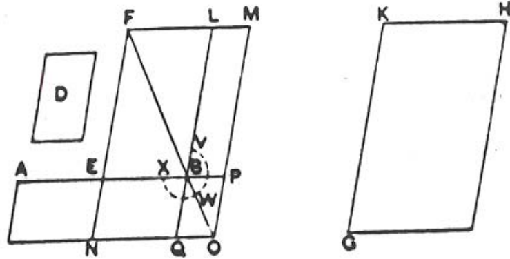
Diagram 4: Book 6, Prop 29
