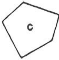
Diagram 4: Book 6, Prop 29
